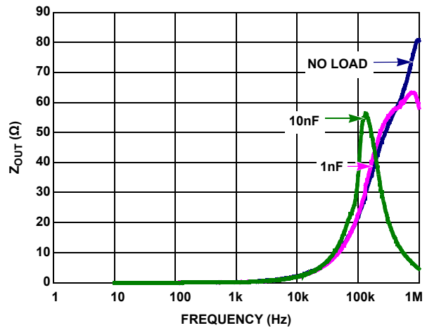
FIGURE 55. Z_{OUT} vs FREQUENCY
