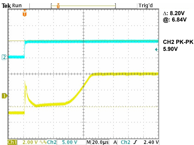
FIGURE 27. TURN-ON TIME, 1k \Omega
